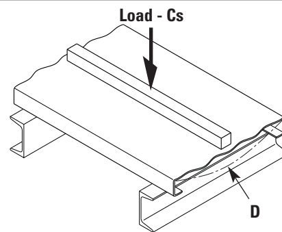
Figure 3 Concentrated Load (Cs) applications to grating surface struts of all walkways/planks: Maximum load (lb./ft.) permitted by flexural stress in grating strut, applied longitudinally to a 1 foot length of grating at midwidth. Deflection (Ds) in all walkways/planks Deflection (in.) corresponding to maximum concentrated strut load (Cs) permitted by flexural stress in grating strut, applied longitudinally to a 1 foot length of grating at midwidth.
